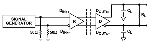
Figure 39. Timing Test Circuit
