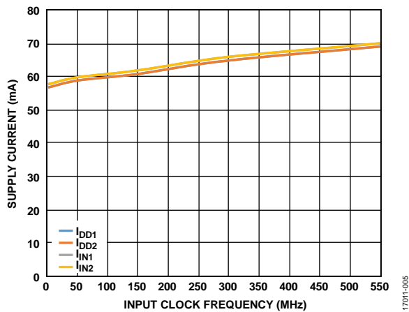
Figure 10. Supply Current vs. Input Clock Frequency ( D_{IN1\pm} and D_{IN2\pm} Switching)
