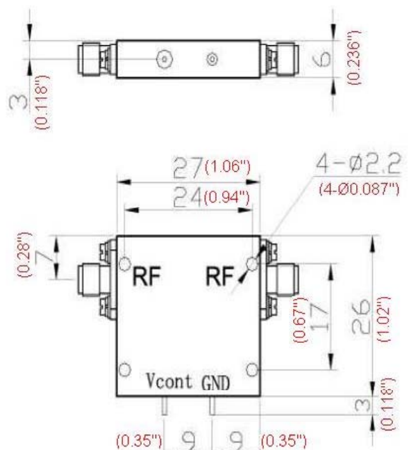
360° Phase Shifter
