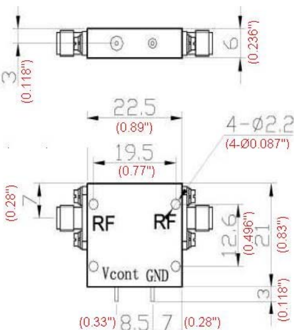
180° Phase Shifter
