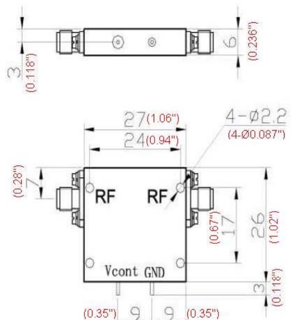
360° Phase Shifter
