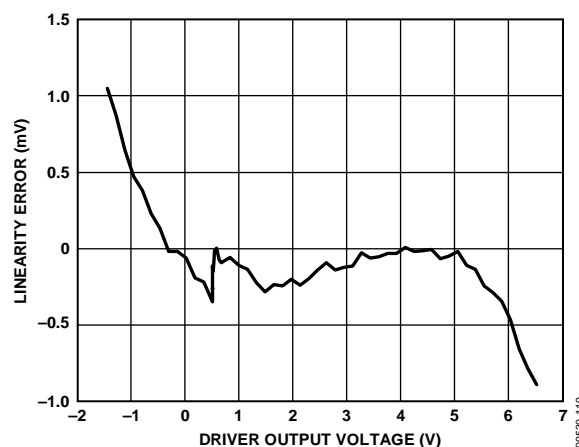
Figure 26. Driver V_{IT} Linearity Error
