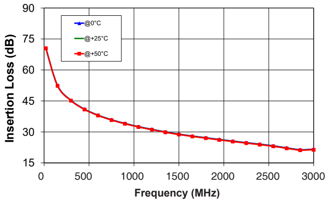
Max Attenuation vs. Frequency
