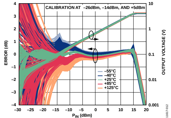
Figure 8. Distribution of Conformance Error with Respect to Output Voltage ( V_{OUT} ) at 25°C vs. RF Input Power ( P_{IN} ) for Various Temperatures at 0.5 GHz
