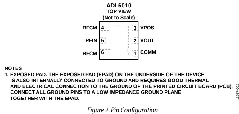
Figure 2. Pin Configuration
