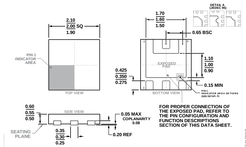
Figure 47. 6-Lead Lead Frame Chip Scale Package [LFCSP] 2.00 mm × 2.00 mm Body and 0.55 mm Package Height (CP-6-7)
