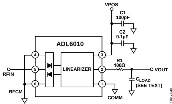
Figure 37. Basic Connections
