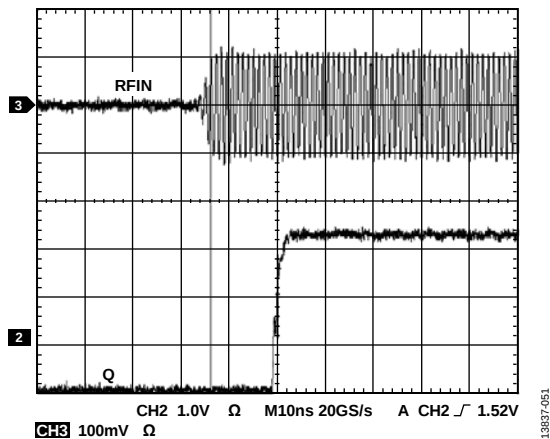
Figure 14. Q Output Response at 900 MHz, P_{IN} = Off to -9 dBm, Overdrive Threshold Voltage Set to Trigger at -10 dBm (Overdrive Level = 1 dB)
