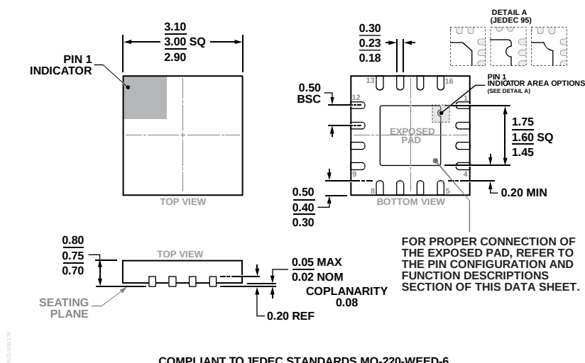
Figure 25. 16-Lead Lead Frame Chip Scale Package [LFCSP]
