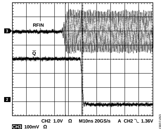
Figure 16. \bar{Q} Output Response, P_{IN} = Off to -7 dBm, Overdrive Threshold Voltage Set to Trigger at -10 dBm (Overdrive Level = 3 dB)
