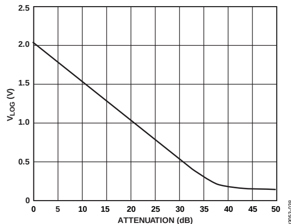
Figure 39. Example of an Absorbance Transfer Function
