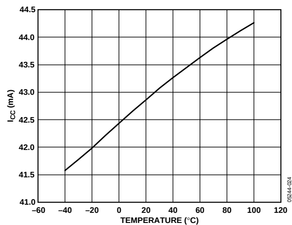
Figure 19. ADN2891 I CC Current vs. Temperature
