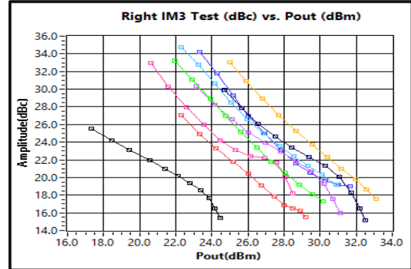
Right IM3 vs. Output Power 28GHz-40GHz
