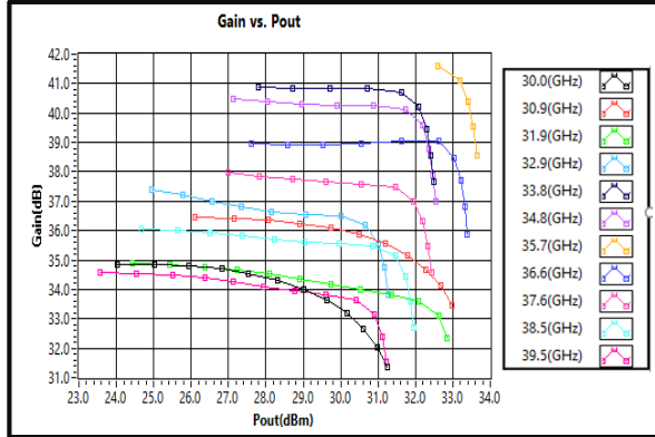
Gain vs. Output Power 30GHz-40GHz
