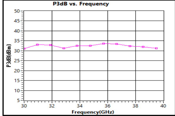
P3dB vs. Frequency 30GHz-40GHz
