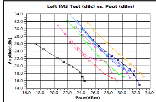
Left IM3 vs. Output Power 28GHz-40GHz
