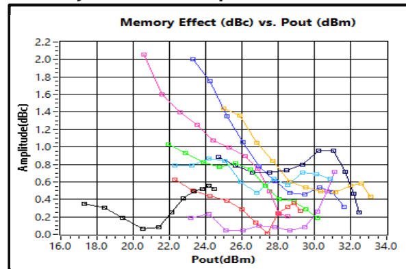
Memory Effect vs. Output Power 28GHz-40GHz
