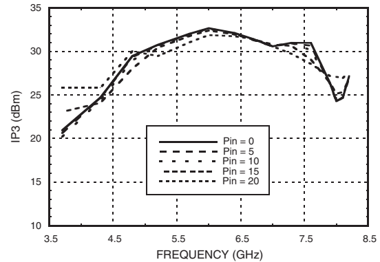
Input IP3 vs. Power Input V_{ctl} = V_{bwctl}
