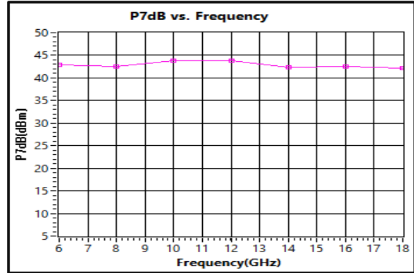
P7dB vs. Frequency 6GHz-18GHz
