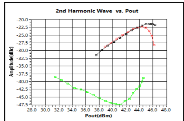
2nd Harmonic Wave Output Power 6-18GHz
