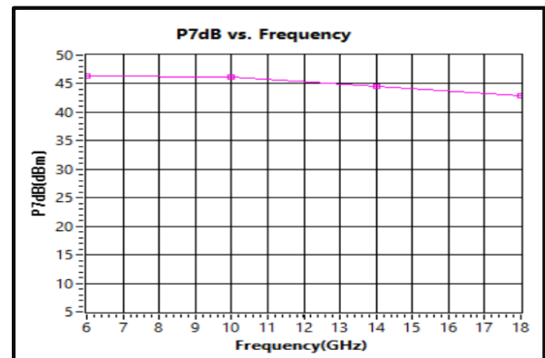
P7dB vs. Frequency 6-18GHz
