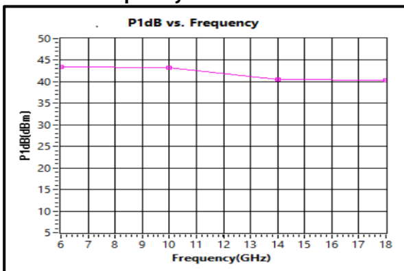
P1dB vs. Frequency 6-18GHz
