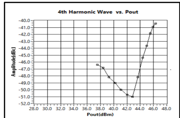
4th Harmonic Wave output Power 6-10GHz
