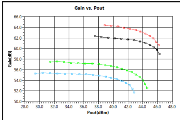
Gain vs. Output Power 6-18GHz
