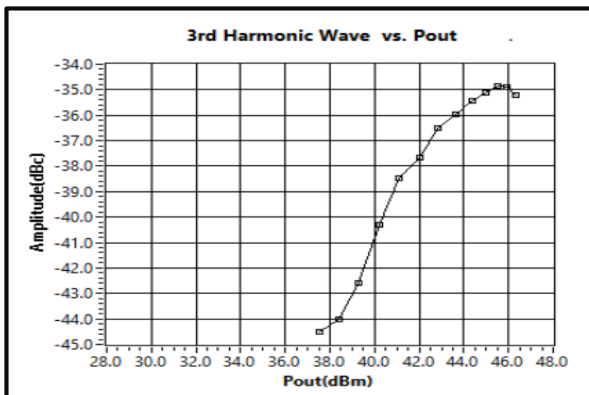
3rd Harmonic Wave output Power 6-18GHz
