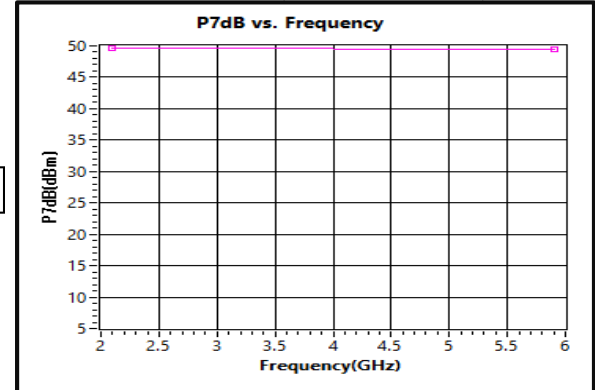
P7dB vs Frequency (2.1 and 5.9GHz)
