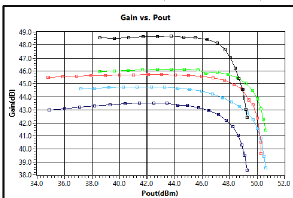
Gain vs Output Power (2GHz to 6GHz)
