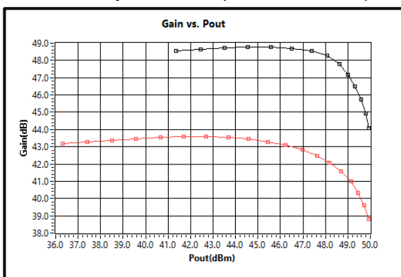
Gain vs Output Power (2.2 and 5.8GHz)
