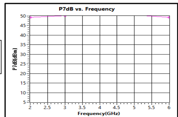
P7dB vs Frequency (2GHz to 6GHz)
