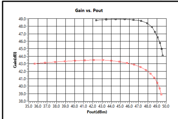
Gain vs Output Power (2.1 and 5.9GHz)
