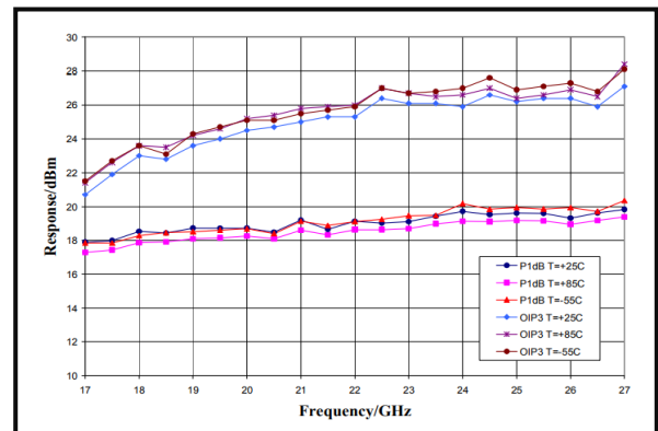
P1dB & Output IP3 vs. Temperature
