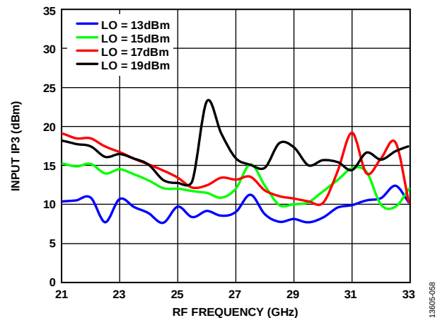
Figure 60. Input IP3 vs. RF Frequency at Various LO Powers, T_A = 25^\circ\text{C}
