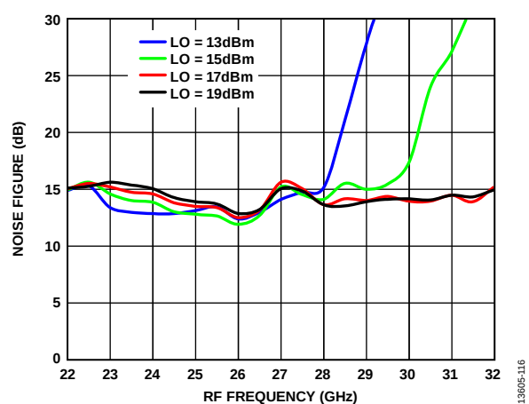
Figure 16. Noise Figure vs. RF Frequency at Various LO Powers, T_A = 25^\circ\text{C}
