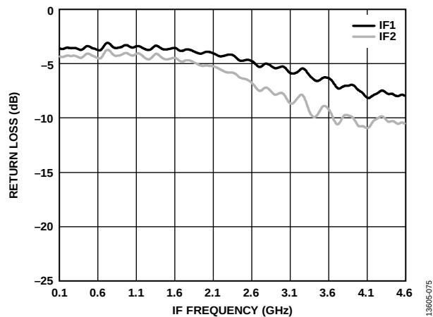
Figure 79. Return Loss vs. IF Frequency, LO = 17 dBm at 27 GHz, T_A = 25^\circ\text{C}
