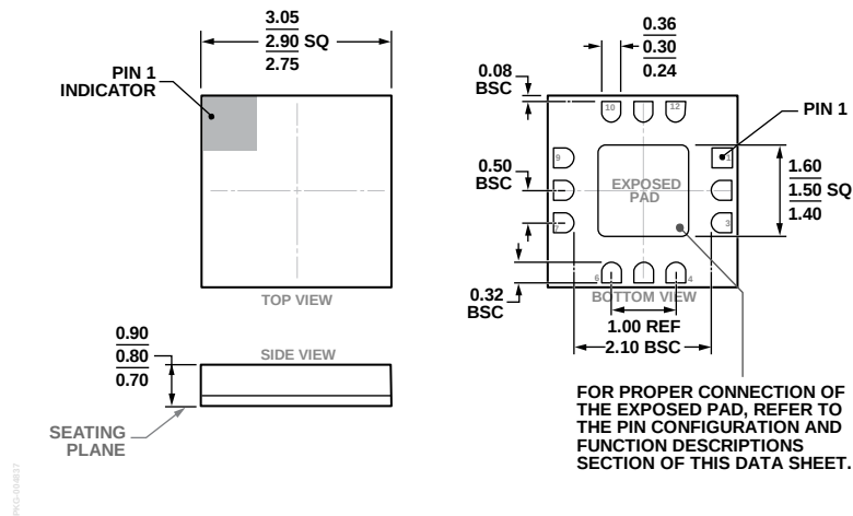
Figure 83. 12-Terminal Ceramic Leadless Chip Carrier (LCC) (E-12-4)
