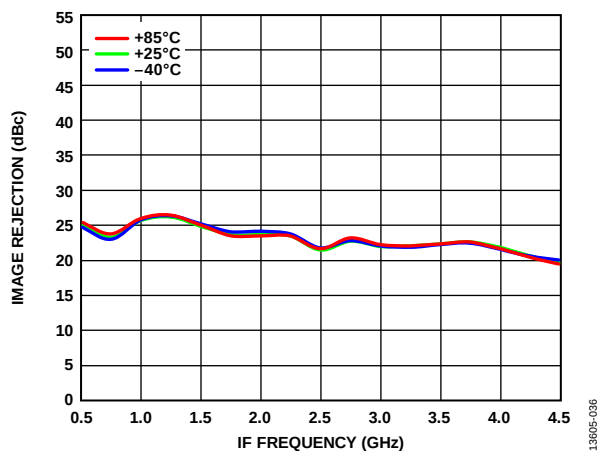
Figure 38. Image Rejection vs. IF Frequency at Various Temperatures
