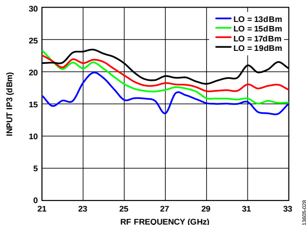
Figure 30. Input IP3 vs. RF Frequency at Various LO Powers, T_A = 25^\circ\text{C}
