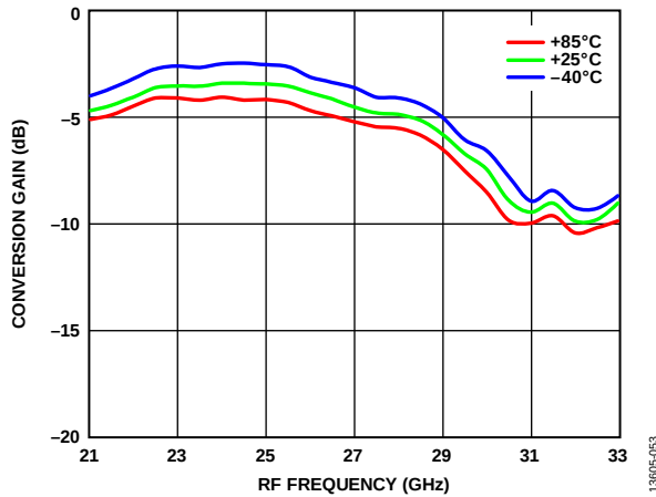
Figure 55. Conversion Gain vs. RF Frequency at Various Temperatures
