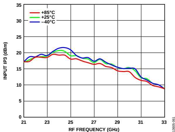
Figure 63. Input IP3 vs. RF Frequency at Various Temperatures
