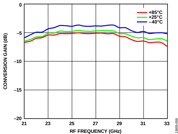
Figure 61. Conversion Gain vs. RF Frequency at Various Temperatures
