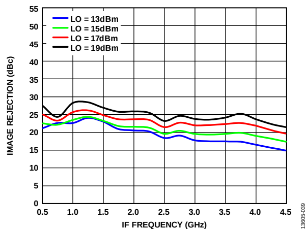
Figure 41. Image Rejection vs. IF Frequency at Various LO Powers, T_A = 25^\circ\text{C}
