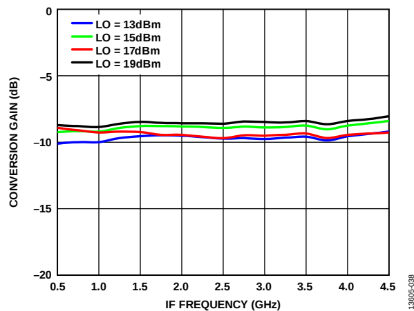
Figure 40. Conversion Gain vs. IF Frequency at Various LO Powers, T_A = 25^\circ\text{C}
