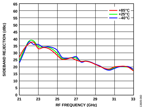
Figure 62. Sideband Rejection vs. RF Frequency at Various Temperatures
