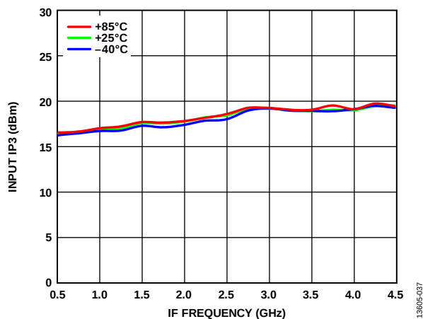
Figure 39. Input IP3 vs. IF Frequency at Various Temperatures
