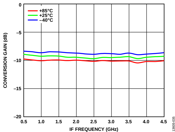
Figure 37. Conversion Gain vs. IF Frequency at Various Temperatures
