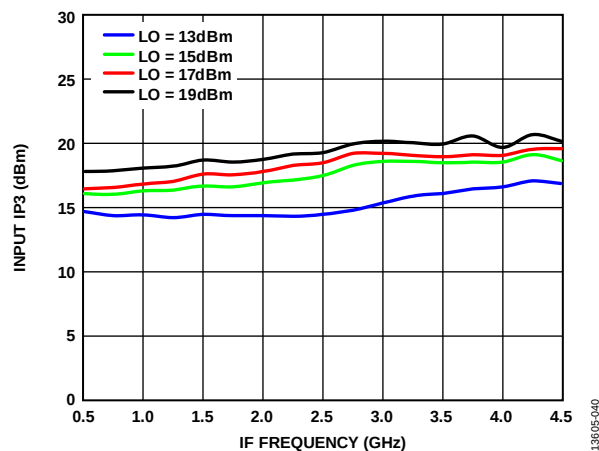
Figure 42. Input IP3 vs. IF Frequency at Various LO Powers, T_A = 25^\circ\text{C}
