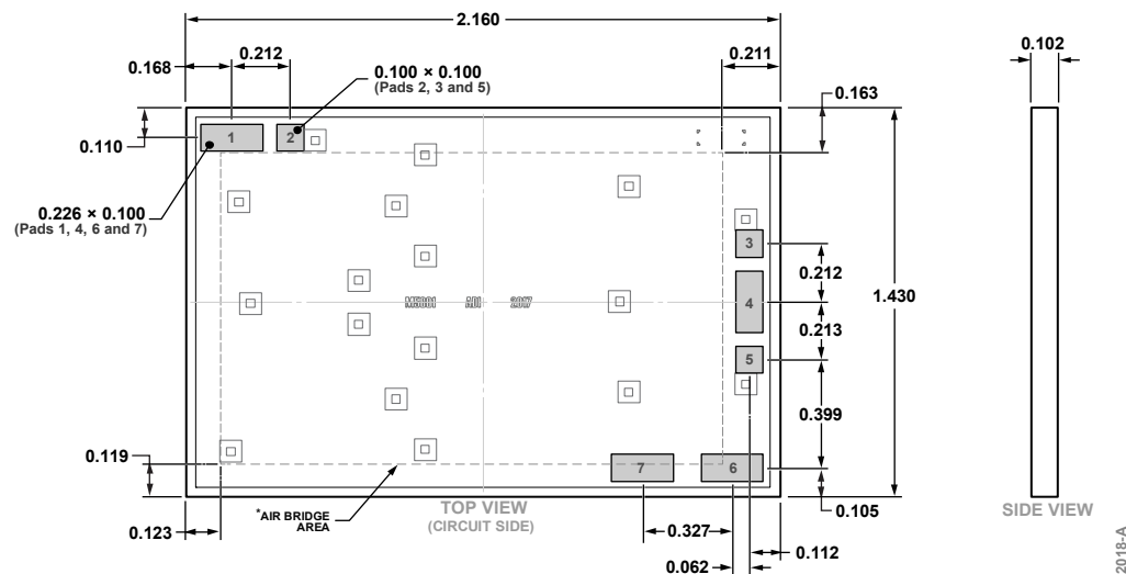
Figure 52. 7-Pad Bare Die [CHIP] (C-7-6)
