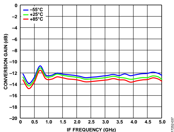
Figure 37. Conversion Gain vs. IF Frequency at Various Temperatures, LO Drive = 18 dBm at 32 GHz
