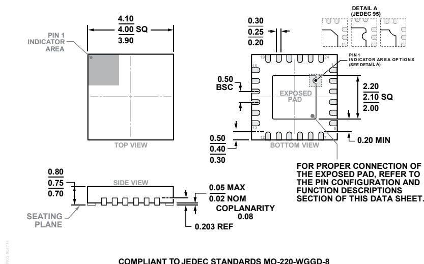
Figure 45. 24-Lead Lead Frame Chip Scale Package [LFCSP] 4 mm × 4 mm Body and 0.75 mm Package Height (CP-24-10)
