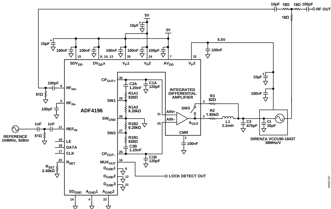
Figure 37. LO for DCS1800 Tx Using the ADF4196
