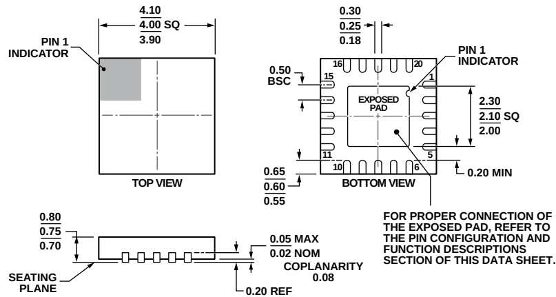
Figure 27. 20-Lead Lead Frame Chip Scale Package [LFCSP_WQ] 4 mm × 4 mm Body, Very Very Thin Quad (CP-20-6)
