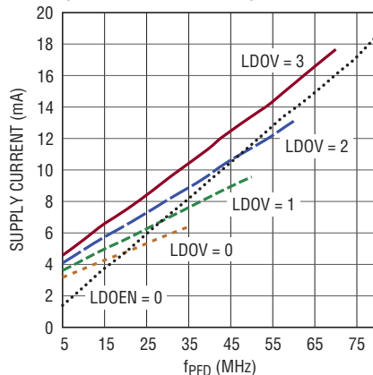
V_D^+ Supply Current vs LDOV, f_{\text{PFD}} ( \text{INTN} = 0 , \text{PDFN} = 0 )
