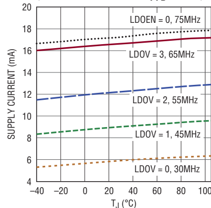
V_D^+ Supply Current vs LDOV, Temperature ( \text{INTN} = 0 , \text{PDFN} = 0 , f_{\text{PFD}} Noted)
