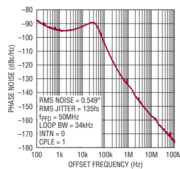
System Phase Noise, f_{RF} = 11.260\text{GHz}
