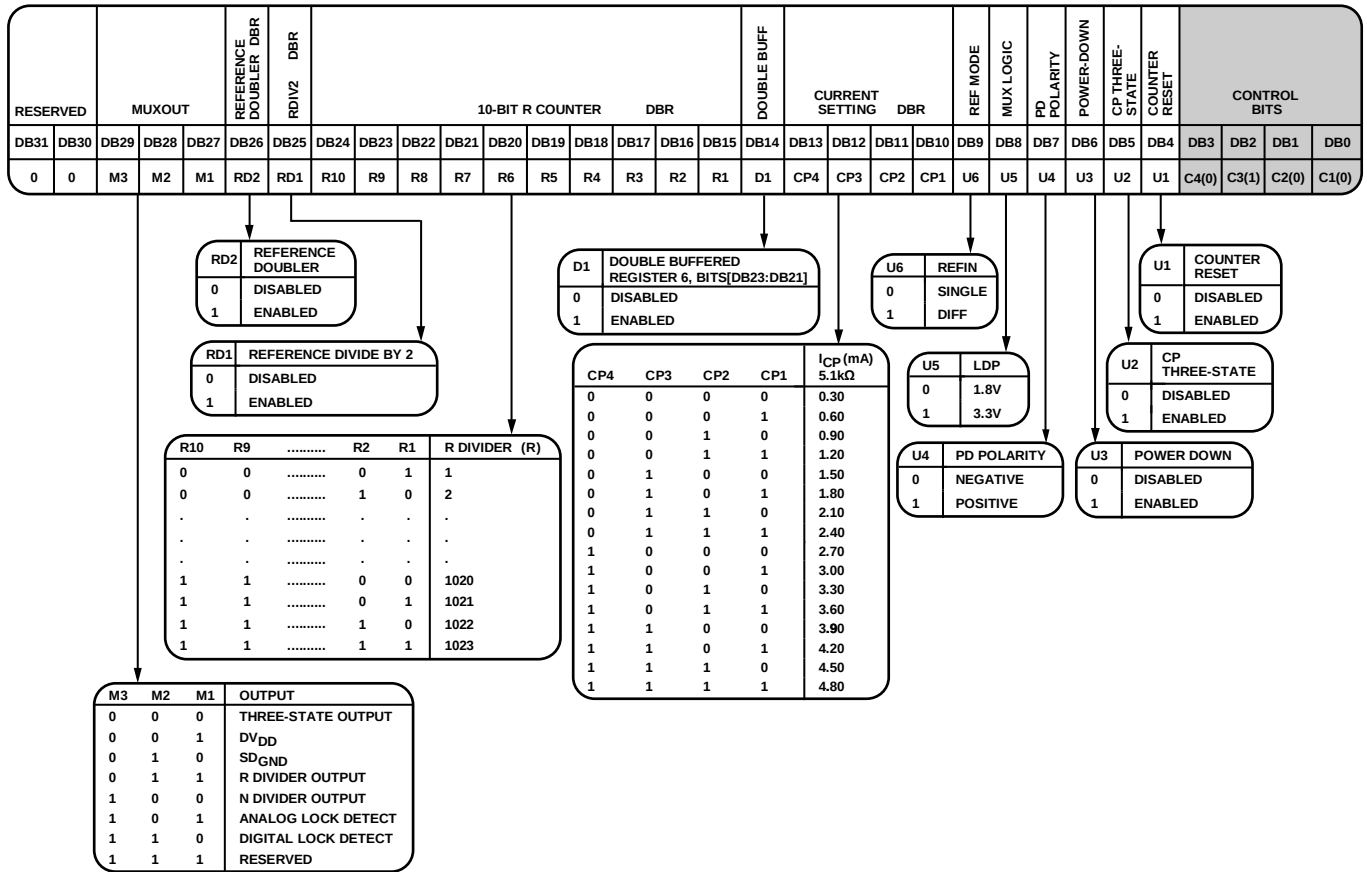
Figure 32. Register 4
