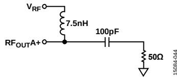
Figure 44. Optimum Output Stage
