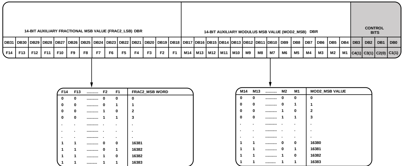
Figure 41. Register 13
