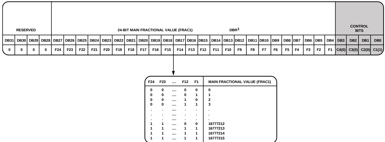
Figure 29. Register 1
