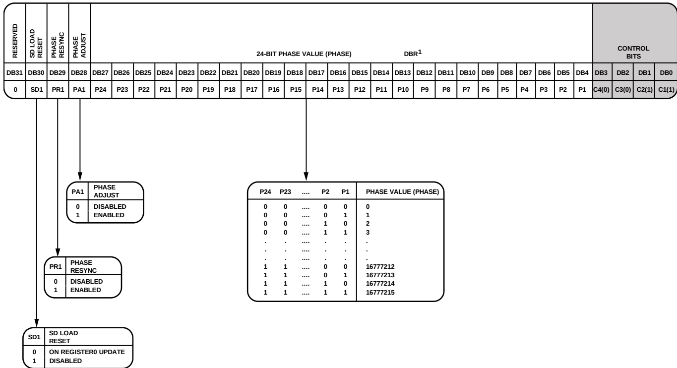
Figure 31. Register 3
