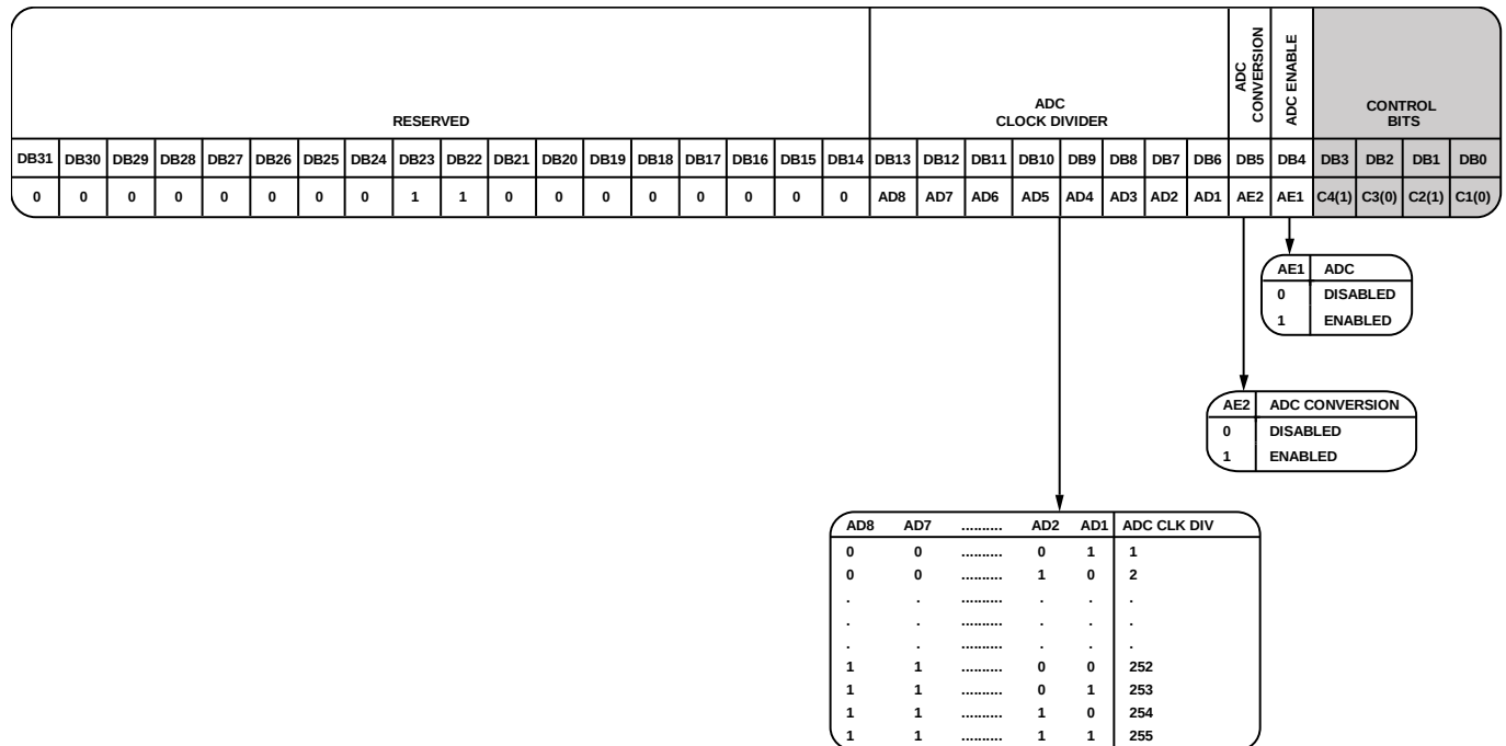
Figure 38. Register 10
