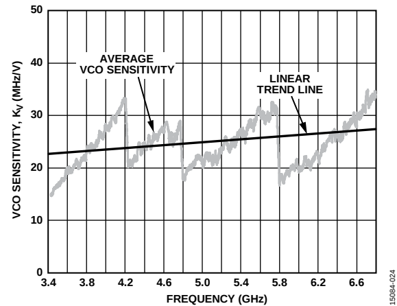
Figure 24. VCO Sensitivity, K_V vs. Frequency
