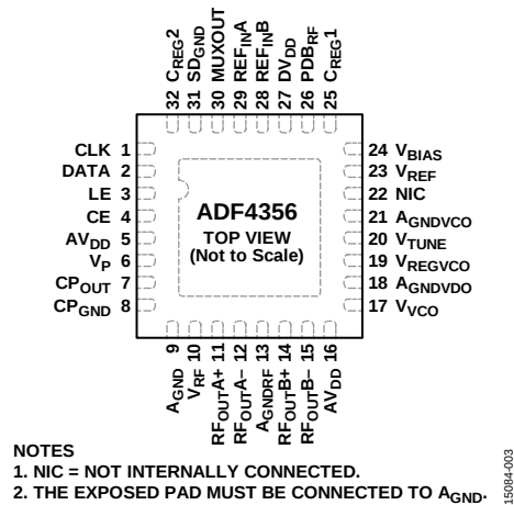
Figure 3. Pin Configuration
