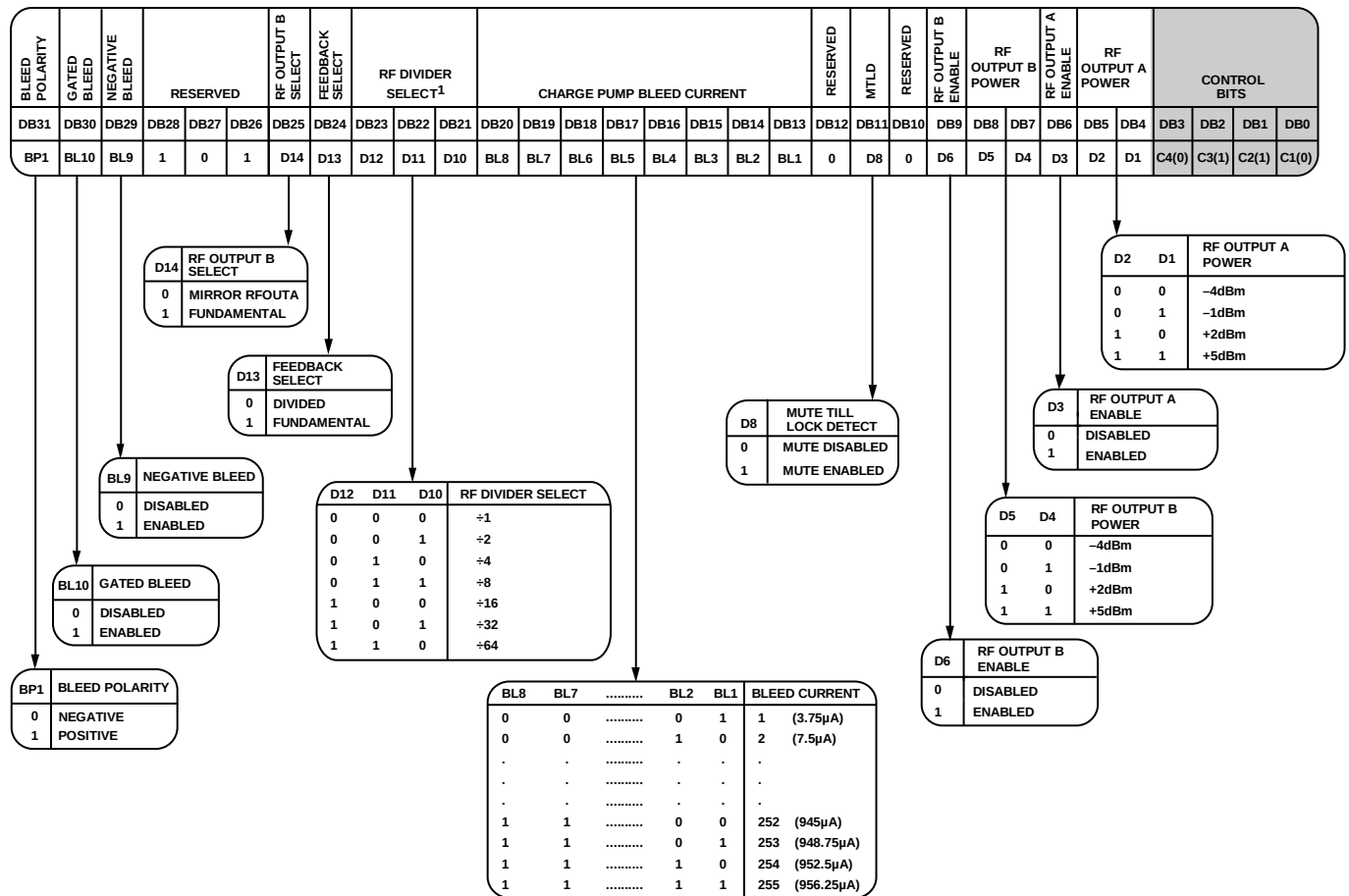
Figure 34. Register 6
