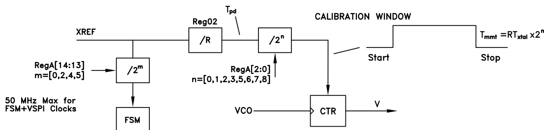
A 5-bit step tuned VCO, for example, nominally requires 5 measurements for calibration, worst case 6 measurements, and hence 7 VSPI data transfers of 20 clock cycles each. The measurement has a programmable number of wait states, k, of 100 FSM cycles defined by Reg 0Ah[7:6] = k. Hence total calibration time, worst case, is given by:
