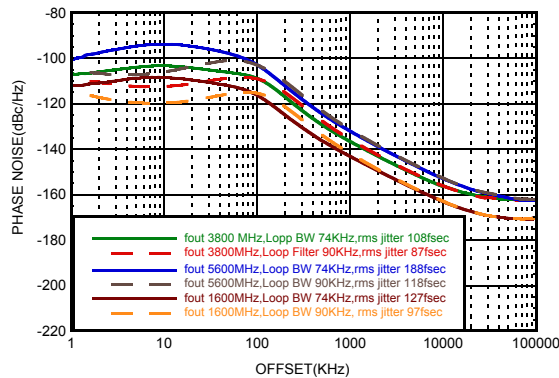
Figure 1. Typical Closed Loop Integer Phase Noise [1] Loop Filter Configuration Table
