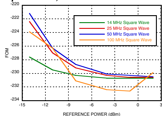
Figure 11. Reference Input Sensitivity, Square Wave, 50 \Omega [3]
