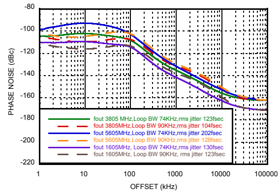
Figure 2. Typical Closed Loop Fractional Phase Noise [1] Loop Filter Configuration Table
