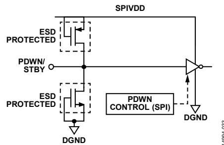
Figure 54. PDWN/STBY Input
