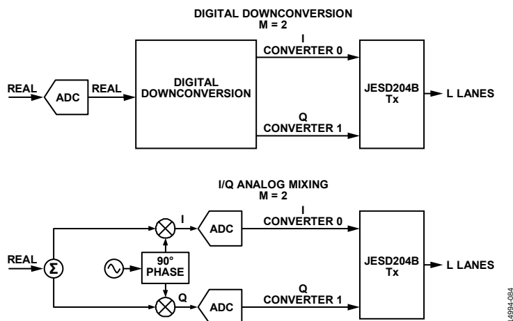
Figure 97. I/Q Transport Layer Mapping
