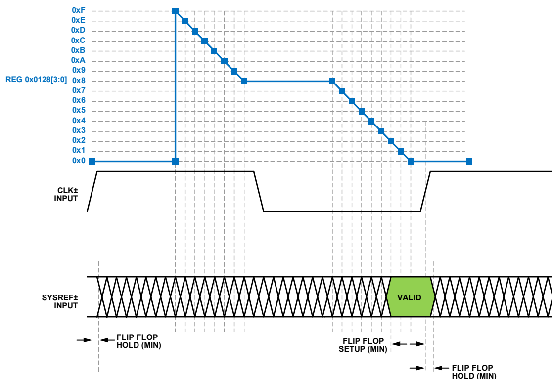
Figure 102. SYSREF± Setup Detector
