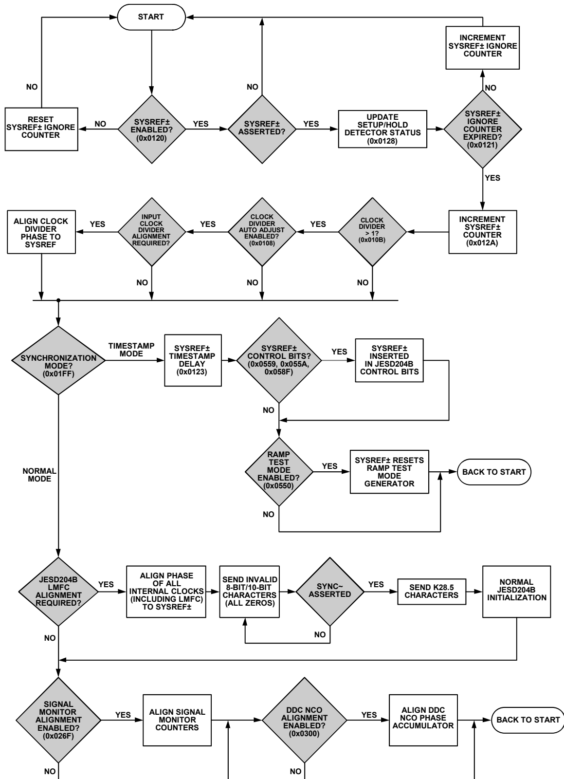
Figure 101. Multichip Synchronization
