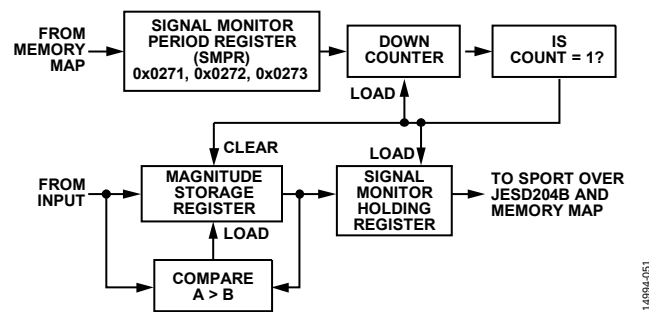
Figure 69. Signal Monitor Block
