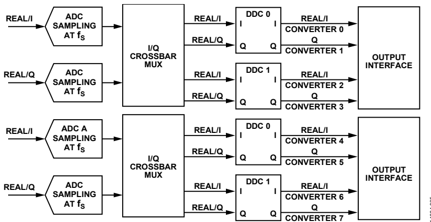
Figure 98. DDCs and Virtual Converter Mapping
