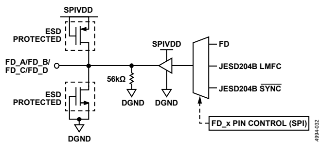
Figure 53. FD_A/FD_B/FD_C/FD_D Outputs
