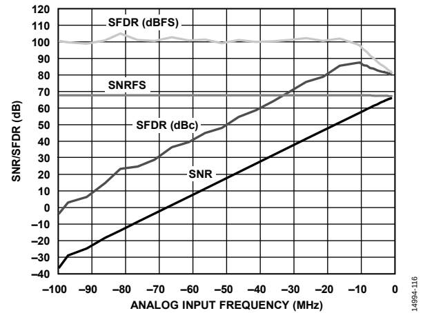
Figure 22. SNR/SFDR vs. Analog Input Frequency, f_{IN} = 305\text{ MHz}
