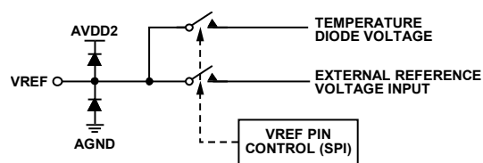
Figure 55. VREF Input/Output
