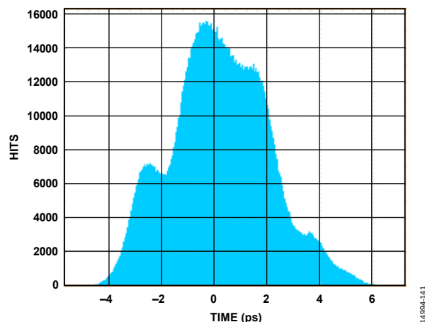
Figure 95. AD6684 Digital Outputs Histogram; External 100 \Omega Terminations at 15 Gbps
