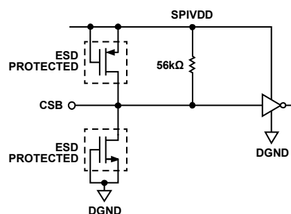
Figure 51. CSB Input
