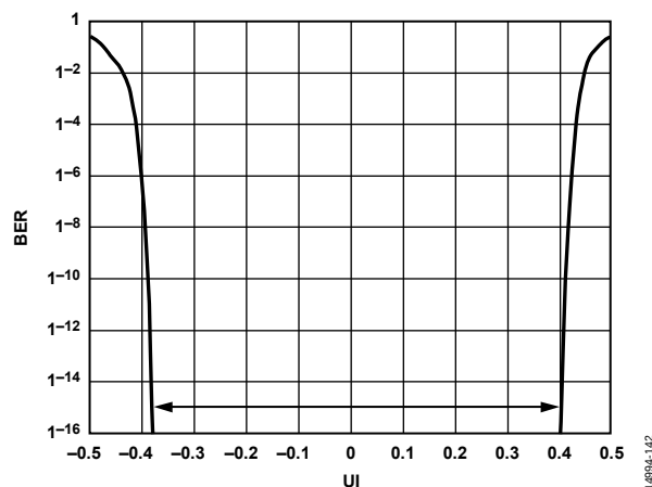
Figure 96. AD6684 Digital Outputs Bathtub Curve; External 100 \Omega Terminations at 15 Gbps
