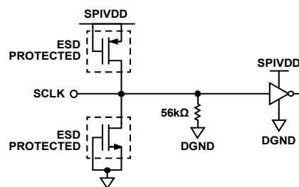
Figure 50. SCLK Input
