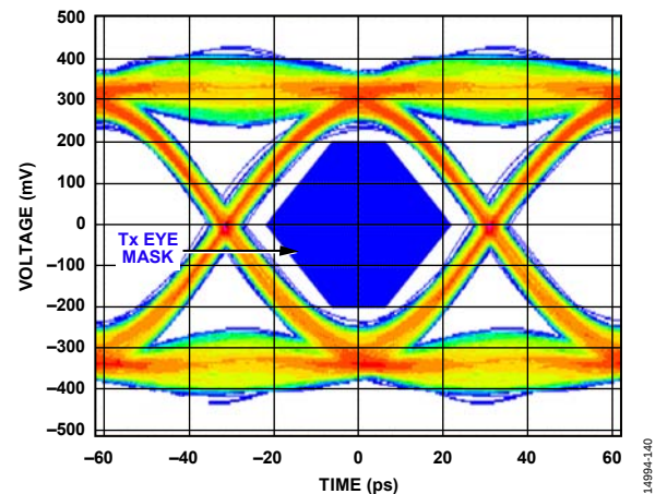
Figure 94. AD6684 Digital Outputs Data Eye Diagram; External 100 \Omega Terminations at 15 Gbps
