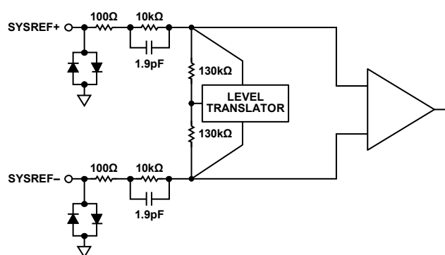
Figure 47. SYSREF± Inputs
