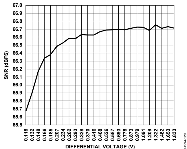
Figure 35. SNR vs. Clock Amplitude (Differential Voltage), f_{IN} = 155.3 MHz
