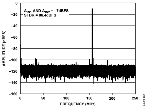
Figure 18. Two Tone FFT; f_{IN1} = 153.5\text{ MHz} , f_{IN2} = 156.5\text{ MHz}
