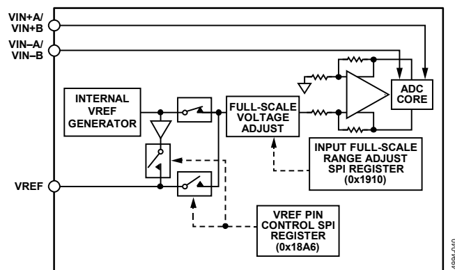
Figure 60. Internal Reference Configuration and Controls
