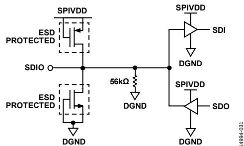
Figure 52. SDIO Input
