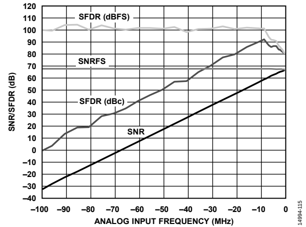
Figure 21. SNR/SFDR vs. Analog Input Frequency, f_{IN} = 155\text{ MHz}
