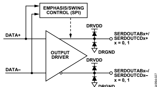
Figure 48. Digital Outputs
