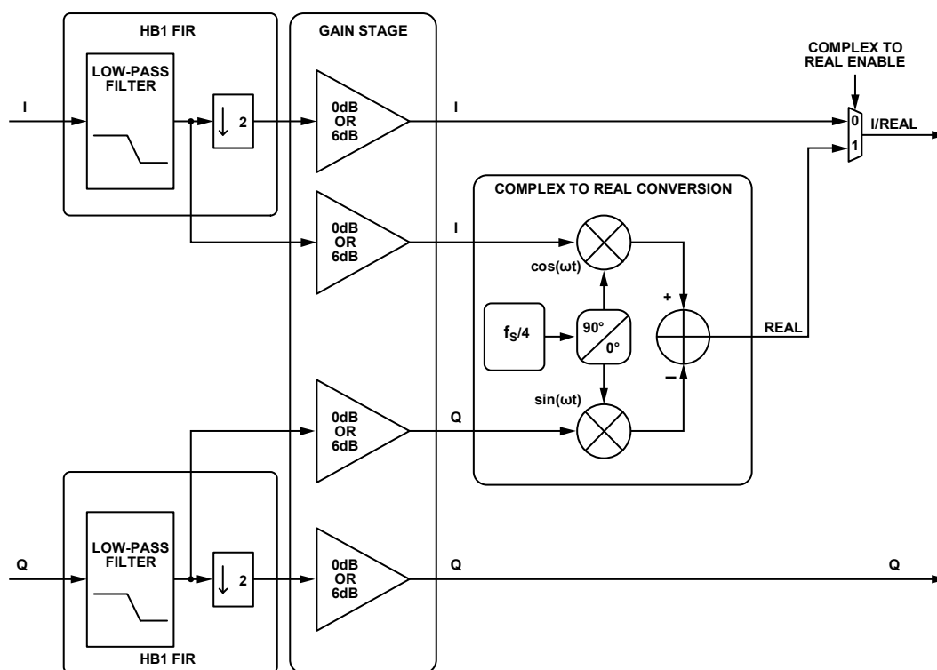
Figure 81. Complex to Real Conversion Block
