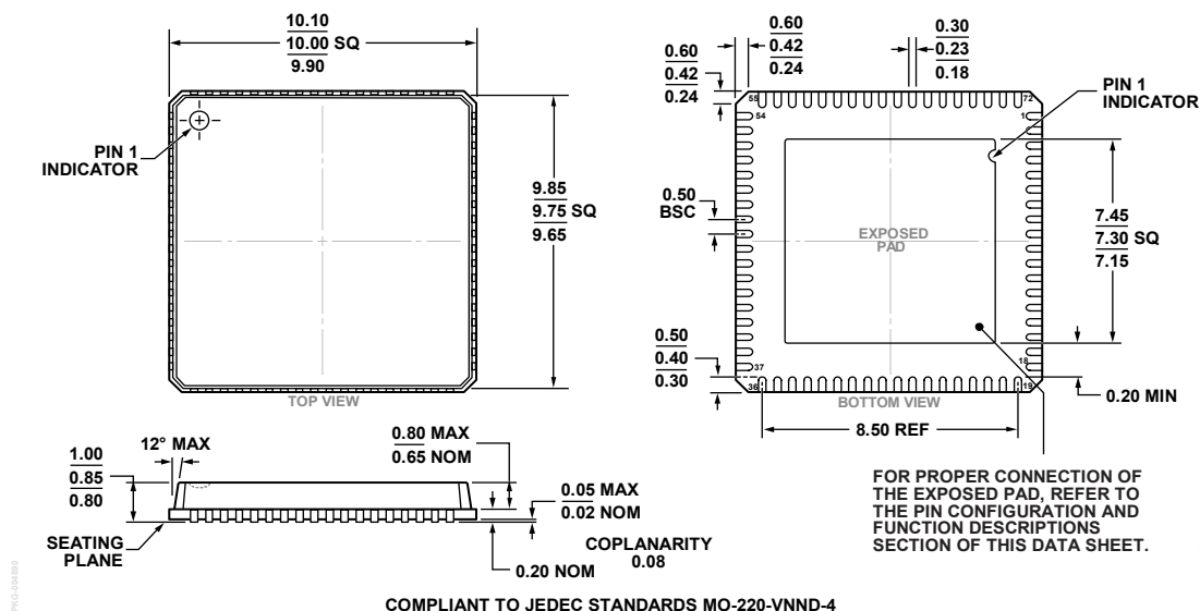
Figure 106. 72-Lead Lead Frame Chip Scale Package [LFCSP] 10 mm × 10 mm Body and 0.85 mm Package Height (CP-72-10) Dimensions shown in millimeters
