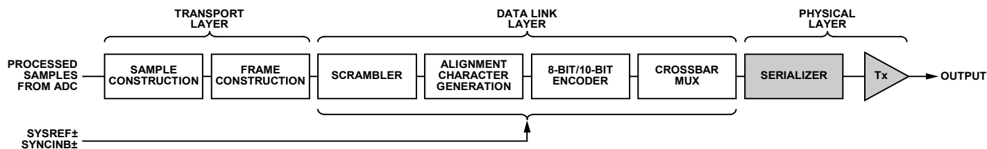
Figure 90. Data Flow
