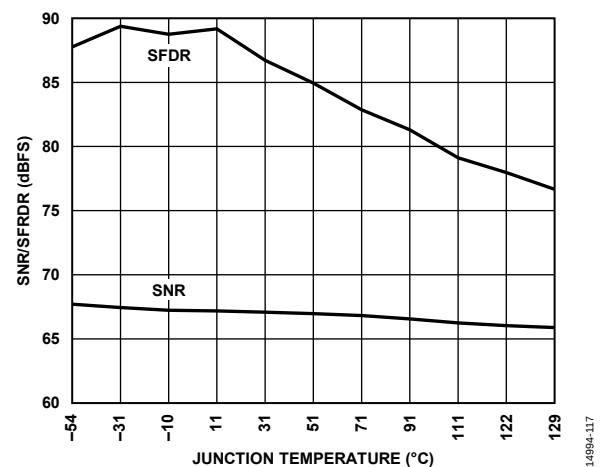
Figure 23. SNR/SFDR vs. Junction Temperature, f_{IN} = 155\text{ MHz}
