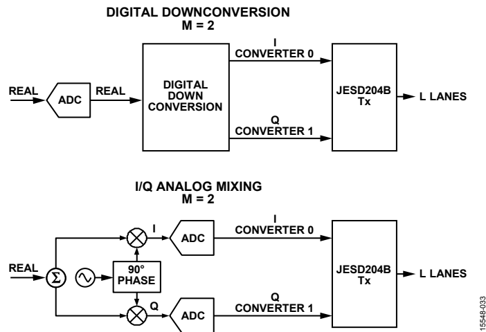
Figure 65. I/Q Transport Layer Mapping
