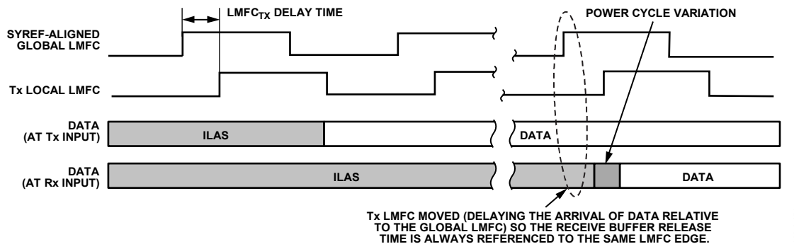
Figure 105. Adjusting the JESD204B Tx LMFC in the AD6688
