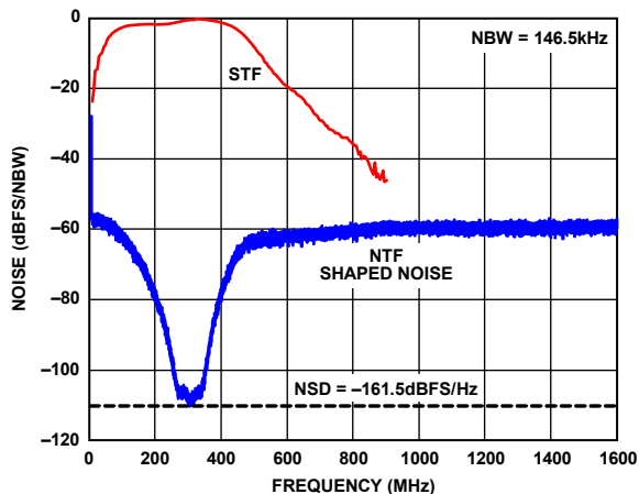
Figure 70. STF and NTF Shaped Noise of the \Sigma - \Delta ADC ( F_{IF} = 300 MHz, BW = 80 MHz, F_{ADC} = 3.2 GHz, L_{EXT} = 19 nH)
