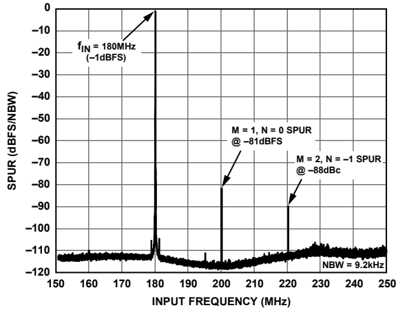
Figure 137. Image Spur for f_{\text{DATA\_IQ}} = 200 MSPS (DEC_MODE = 3) Attributed to M = 2, N = -1
