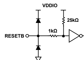
Figure 63. Equivalent RESETB Input Circuit
