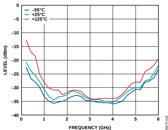
Figure 6. Input Sensitivity
