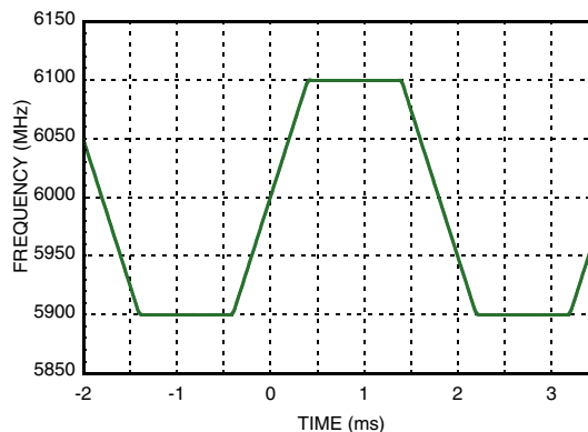
Frequency Sweep
