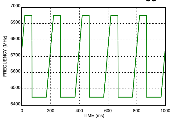
Figure 16. One Way Frequency Sweep, 10 MHz PFD and 10 Hz external trigger [8]
