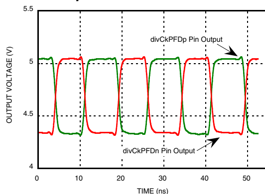
Figure 8. Time Domain 66 MHz Output, 6.5 GHz Input [5]
