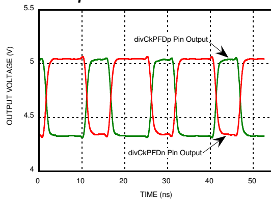
Figure 10. Time Domain 66 MHz Output, 6.5 GHz Input [5]
