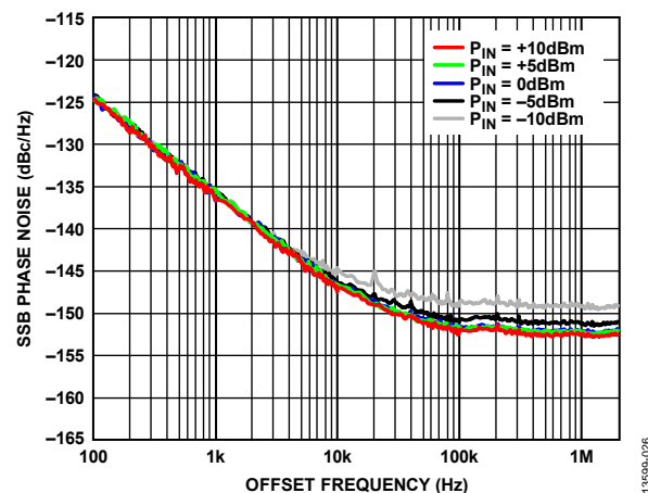
Figure 14. SSB Phase Noise vs. Offset Frequency for Various Input Power ( P_{IN} ) Levels, f_{IN} = 12 GHz Sine Wave, T_A = 25^\circ\text{C}
