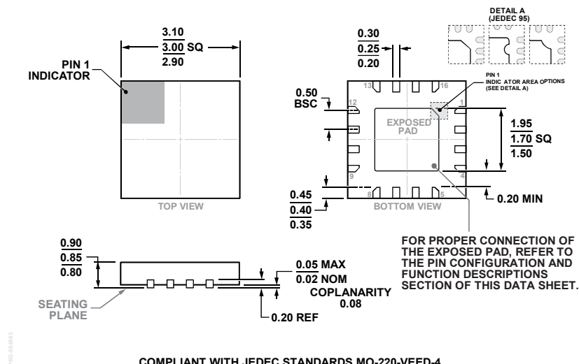
Figure 34. 16-Lead Lead Frame Chip Scale Package [LFCSP] 3 mm x 3 mm Body and 0.85 mm Package Height (HCP-16-1) Dimensions shown in millimeters
