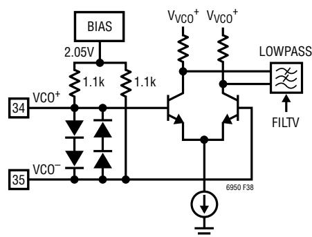
Figure 38. Simplified VCO Input Schematic
