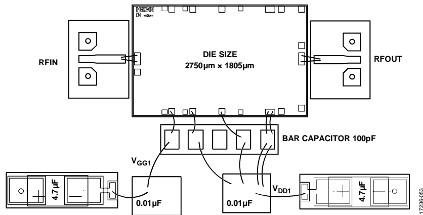
Figure 53. Assembly Diagram
