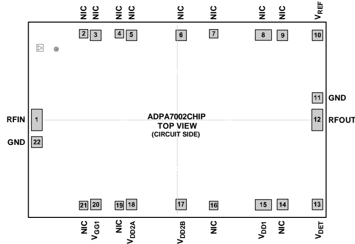
Figure 2. Pin Configuration
