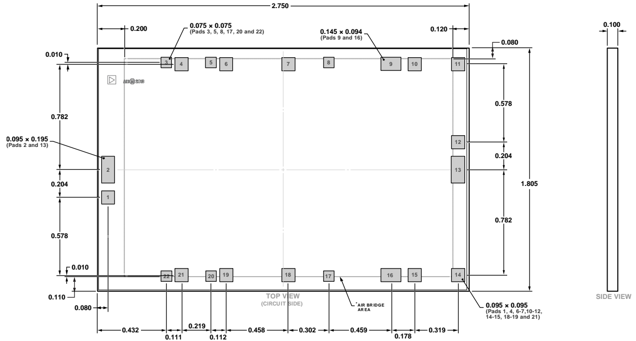
Figure 69. 22-Pad Bare Die [CHIP] (C-22-3)
