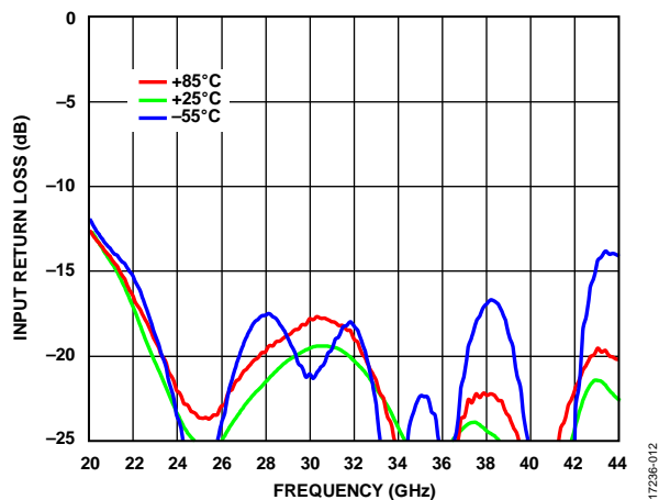
Figure 12. Input Return Loss vs. Frequency for Various Temperatures, V_{DD} = 5\text{ V} , I_{DQ} = 600\text{ mA}
