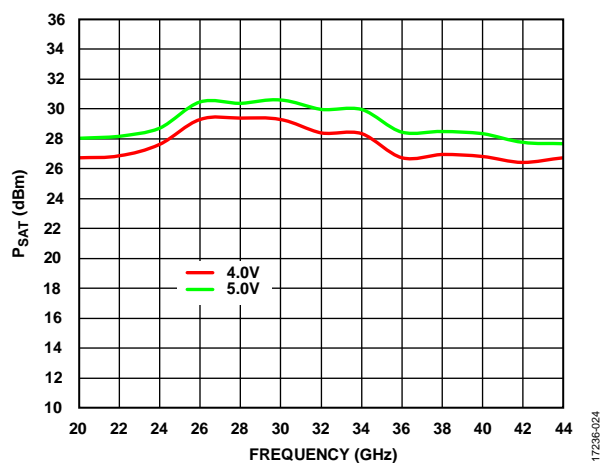
Figure 24. P_{SAT} vs. Frequency for Various Supply Voltages
