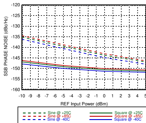
Phase Noise Floor, Vcc = 5.00V REF = 100MHz, ≥10kHz offset
