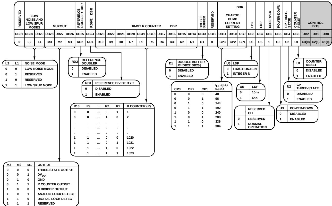
Figure 23. Register 2 (R2)
