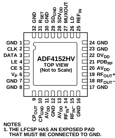
Figure 3. Pin Configuration
