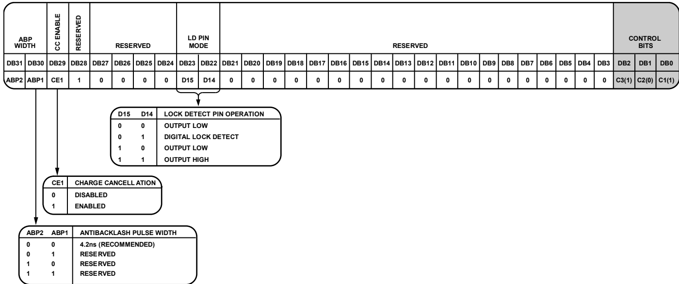
Figure 26. Register 5 (R5)
