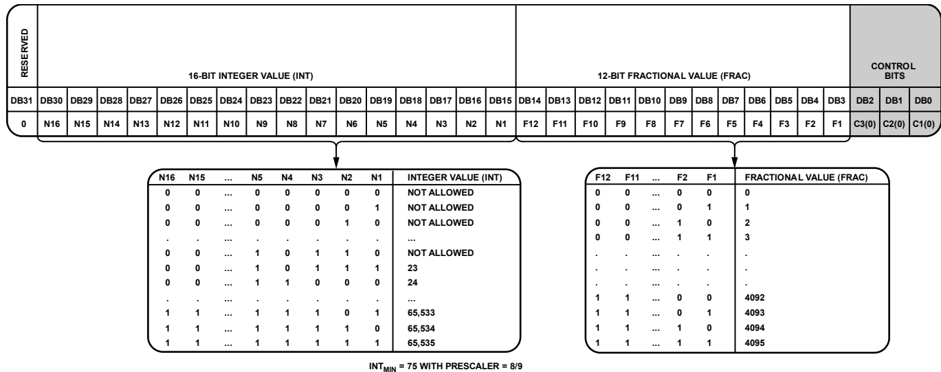
Figure 21. Register 0 (R0)
