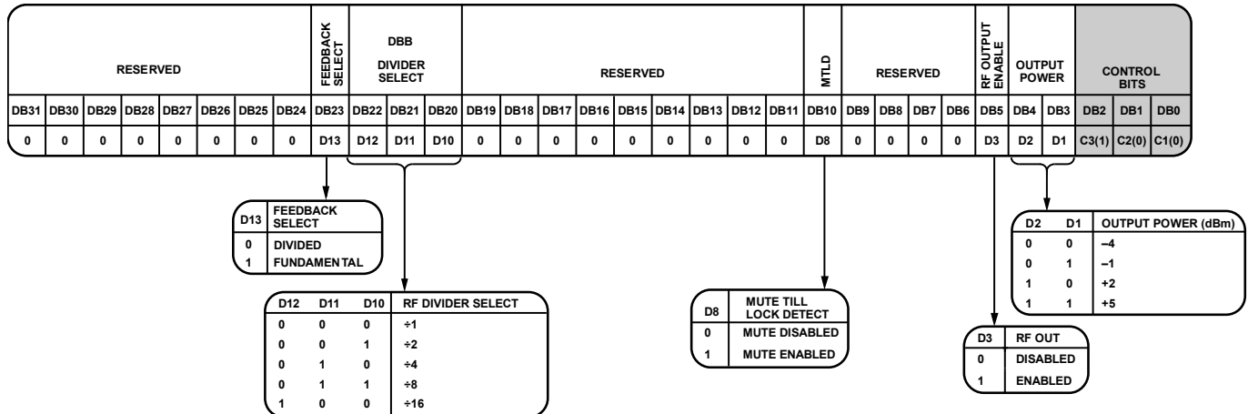
Figure 25. Register 4 (R4)
