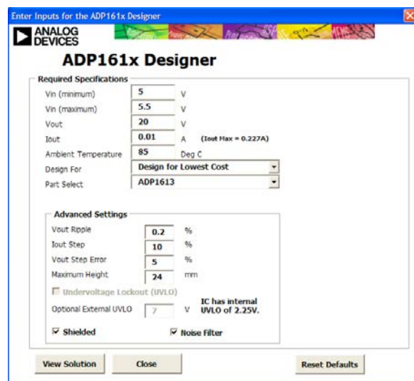
Figure 31. Designer Tool
