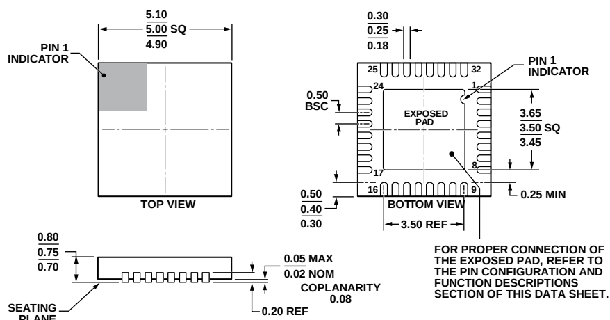
Figure 36. 32-Lead Lead Frame Chip Scale Package [LFCSP] 5 mm × 5 mm Body and 0.75 mm Package Height (CP-32-11)
