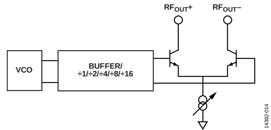
Figure 19. Output Stage
