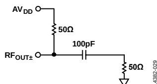
Figure 34. Simple ADF4152HV Output Stage
