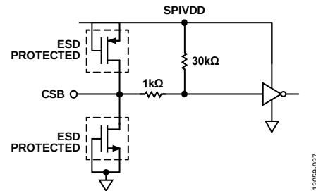
Figure 38. CSB Input
