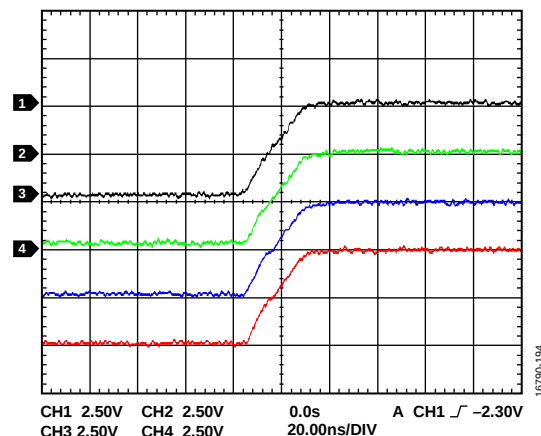
Figure 95. PA_BIAS1, PA_BIAS2, PA_BIAS3, or PA_BIAS4 Rise Time; -10 mA load
