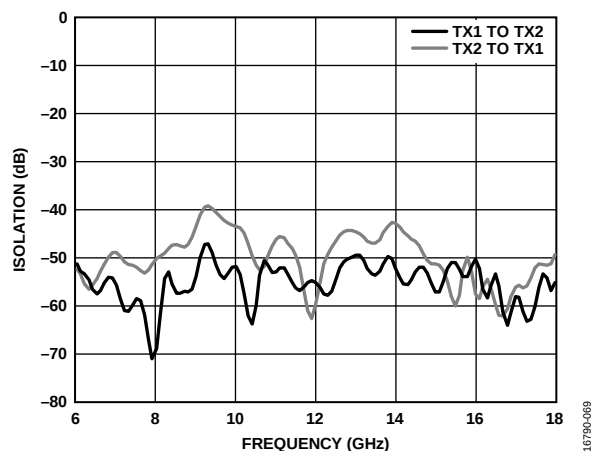
Figure 75. Isolation vs. Frequency, Transmit Channel to Transmit Channel
