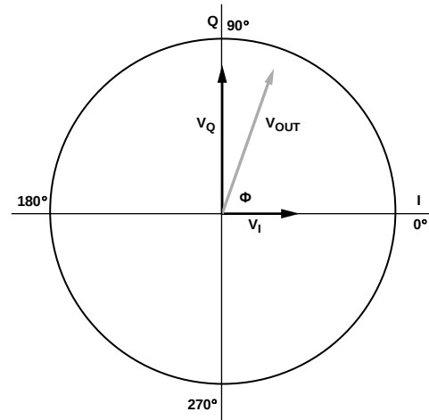
Figure 86. Vector Gain Representation
