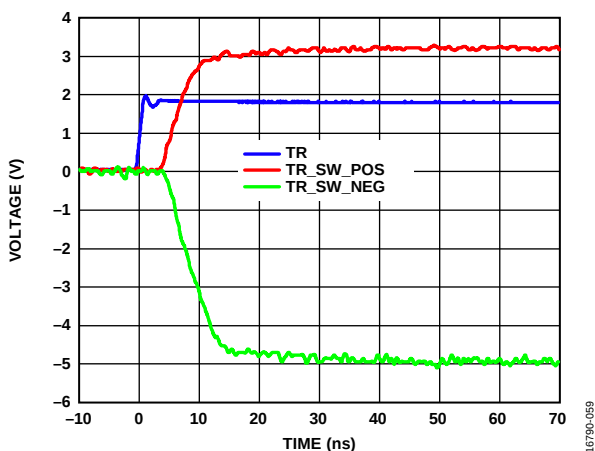
Figure 65. TR_SW_POS and TR_SW_NEG Response to TR Rising Edge
