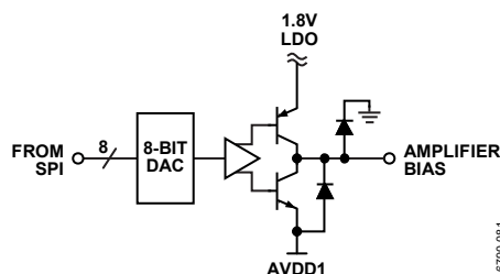
Figure 88. Simplified PA/LNA Bias DAC Schematic
