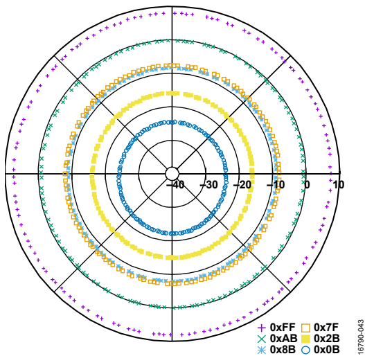
Figure 47. Gain Variation vs. Phase over Gain, 9.5 GHz, Receive Channel
