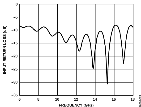
Figure 79. Input Return Loss vs. Frequency, RF Detector
