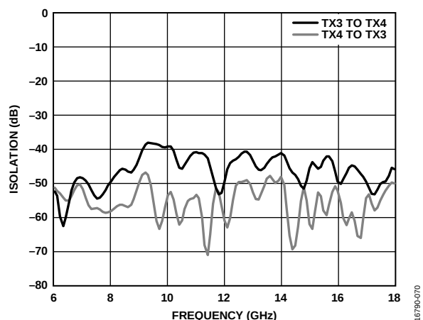
Figure 76. Isolation vs. Frequency, Transmit Channel to Transmit Channel
