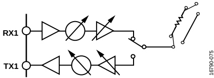
Figure 81. Transmit and Receive Channel Functional Diagram
