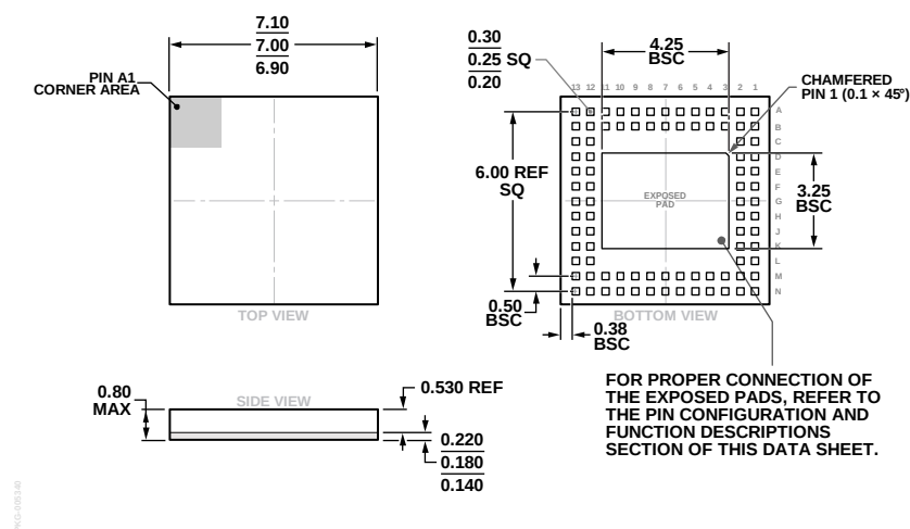
Figure 98. 88-Terminal Land Grid Array [LGA] (CC-88-1) Dimensions shown in millimeters
