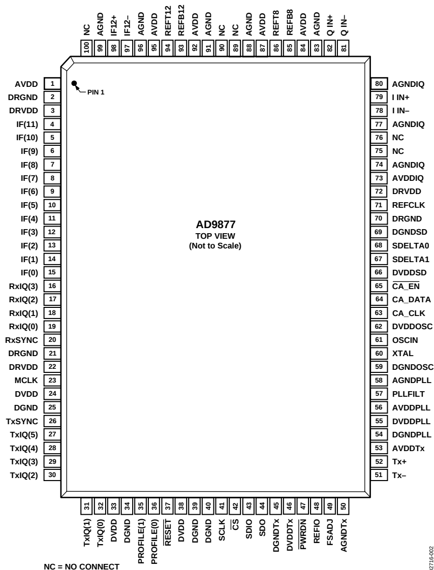
Figure 2. Pin Configuration
