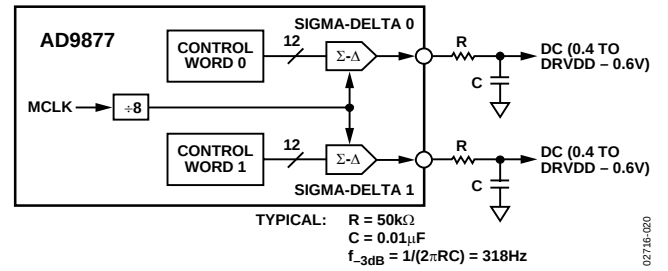
Figure 20. Σ-Δ RC Filter
