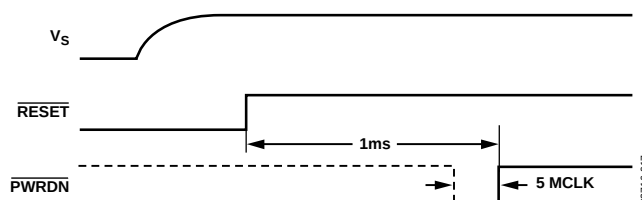
Figure 17. Power-Up Sequence for Tx Data Path
