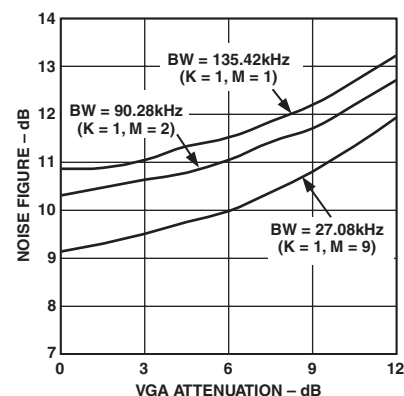
TPC 11c. Noise Figure vs. VGA Attenuation ( f_{CLK} = 26\text{ MSPS} )
