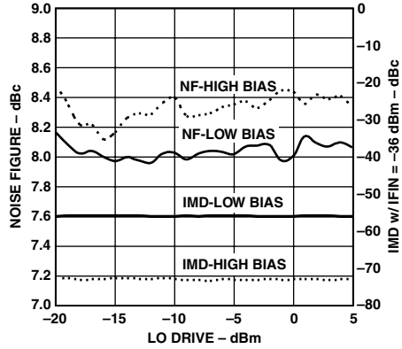
TPC 7b. Noise Figure and IMD vs. LO Drive ( V_{DDx} = 3.0\text{ V} )
