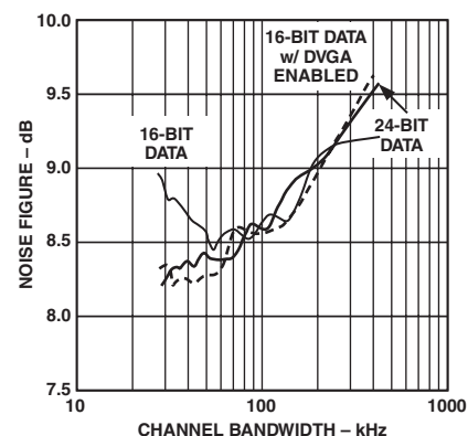
TPC 10c. Noise Figure vs. BW (Minimum Attenuation, f_{CLK} = 26\text{ MSPS} )
