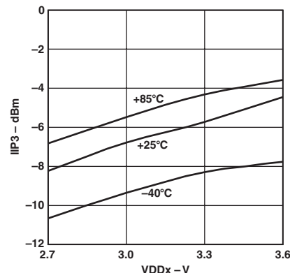
TPC 2c. IIP3 vs. Supply (Low Bias 3 )
