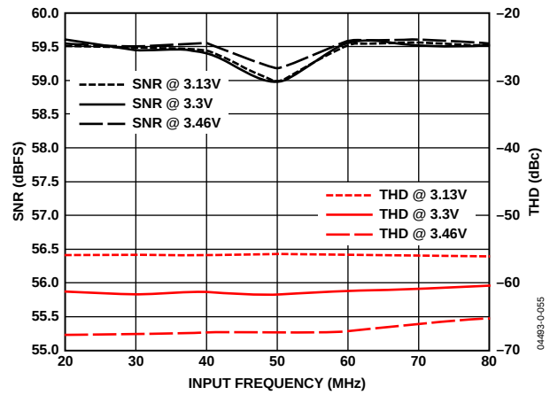
Figure 18. SNR and THD vs. Sample Rate and Supply (LPF Disabled; RxPGA = 0 dB; f_{\text{IN}} = 8 MHz)
