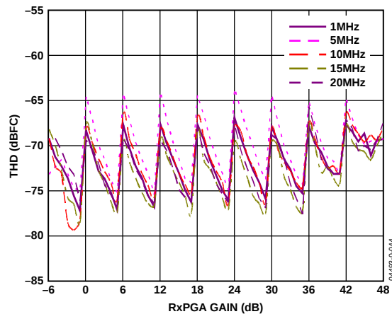
Figure 7. THD vs. R_{\text{xPGA}} Gain and Frequency
