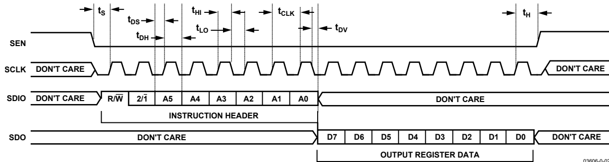
Figure 81. 1-Byte Serial Register Readback in MSB First Mode, SDIO BiDir Bit Set Logic Low (Default, 4-Wire Mode)
