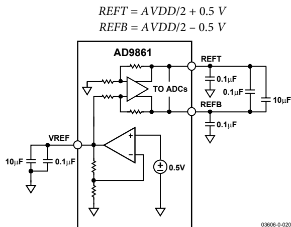
Figure 72. Typical Rx Path Decoupling
