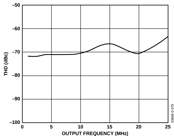
Figure 49. AD9861 Tx Path THD vs. Output Frequency of Tx Path with 2 mA Full-Scale Output into 600 \Omega Differential Load
