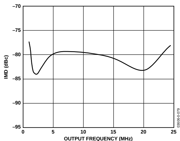
Figure 51. AD9861 Tx Path Dual-Tone (0.5 MHz Spacing) IMD vs. Output Frequency of Tx Path, with 2 mA Full-Scale Output into 600 \Omega Differential Load
