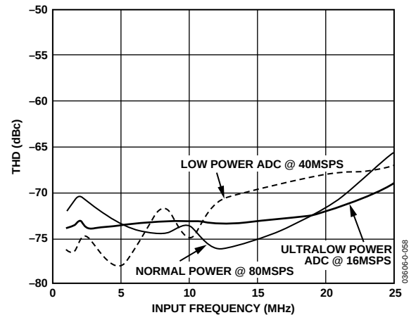
Figure 32. AD9861-80 Rx Path at 80 MSPS, 10 MHz Input Tone THD Performance vs. Input Frequency and Power Setting
