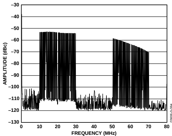
Figure 54. AD9861 Tx Path FFT of OFDM Signal in Figure 52, with 1 \times Interpolation
