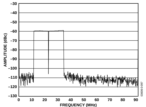
Figure 69. AD9861 Tx Path FFT of OFDM Signal in Figure 52 with 4 \times Interpolation
