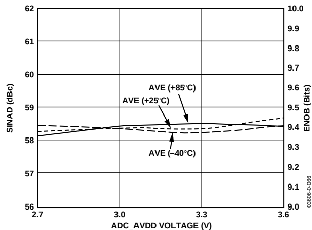
Figure 37. AD9861-80 Rx Path at 80 MSPS, 10 MHz Input Tone SINAD Performance vs. AVDD and Temperature
