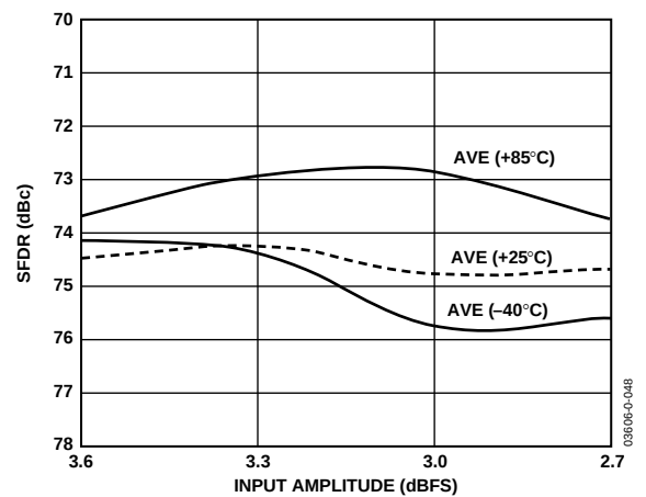
Figure 21. AD9861-50 Rx Path Single-Tone SFDR Performance vs. ADC_AVDD and Temperature
