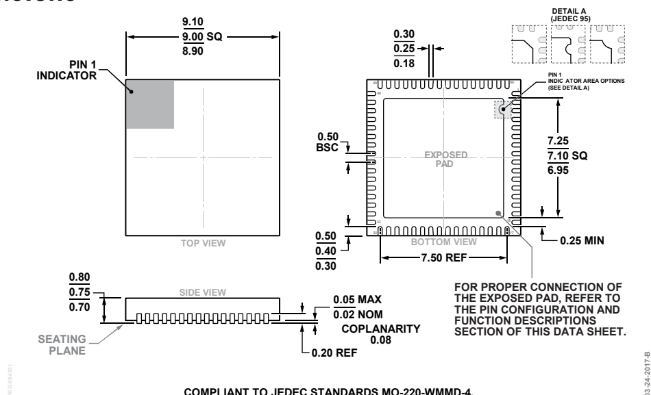
COMPLIANT TO JEDEC STANDARDS MO-220-WMMD-4. Figure 87. 64-Lead Lead Frame Chip Scale Package [LFCSP] 9 mm × 9 mm Body and 0.75 mm Package Height (CP-64-12) Dimensions shown in millimeters
