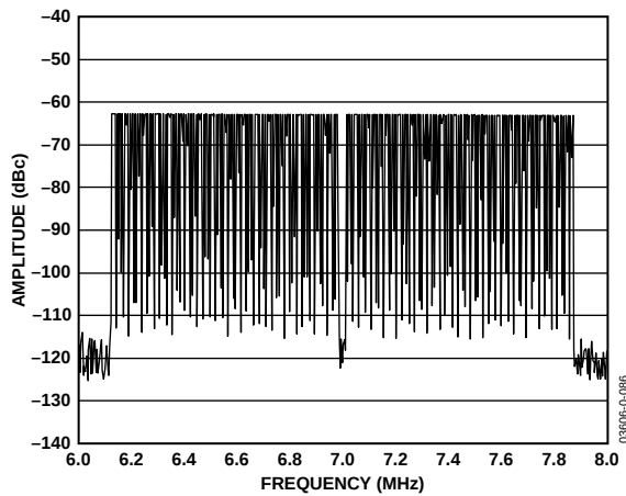
Figure 58. AD9861 Tx Path FFT, 256-Carrier (Center Four Carriers Removed) OFDM Signal over 1.75 MHz Bandwidth, Centered at 7 MHz, with 20 mA Full-Scale Output into 60 \Omega Differential Load
