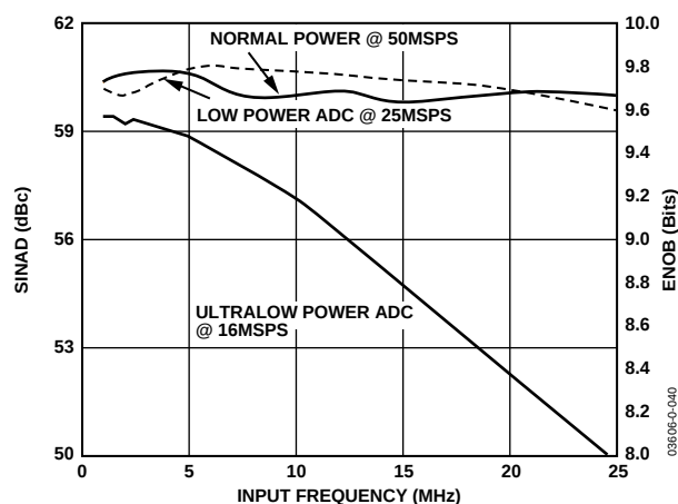
Figure 14. AD9861-50 Rx Path at 50 MSPS, 10 MHz Input Tone SINAD Performance vs. Input Frequency
