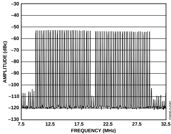
Figure 52. AD9861 Tx Path FFT, 64-Carrier (Center Two Carriers Removed) OFDM Signal over 20 MHz Bandwidth, Centered at 20 MHz, with 20 mA Full-Scale Output into 60 \Omega Differential Load
