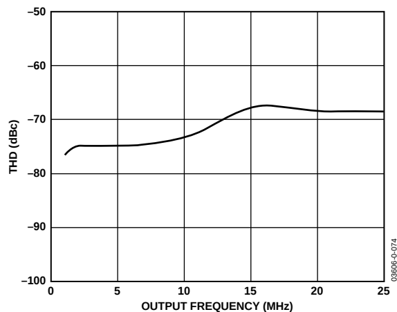
Figure 46. AD9861 Tx Path THD vs. Output Frequency of Tx Path with 20 mA Full-Scale Output into 60 \Omega Differential Load
