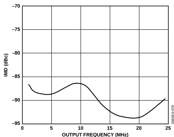
Figure 48. AD9861 Tx Path Dual-Tone (0.5 MHz Spacing) IMD vs. Output Frequency of Tx Path, with 20 mA Full-Scale Output into 60 \Omega Differential Load
