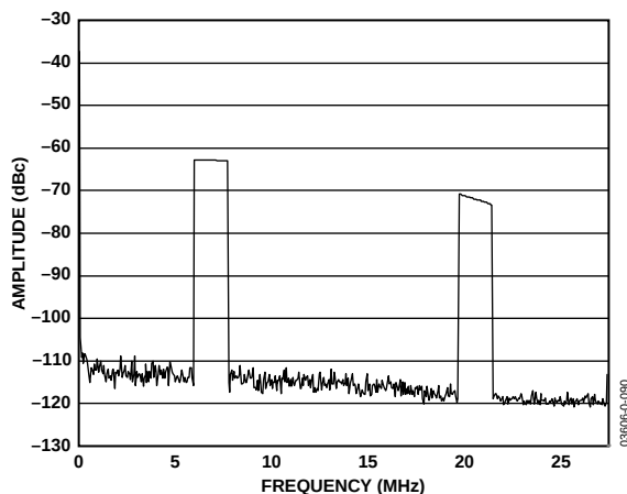
Figure 60. AD9861 Tx Path FFT of OFDM Signal in Figure 52, with 1 \times Interpolation
