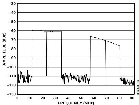
Figure 66. AD9861 Tx Path FFT of OFDM Signal in Figure 52 with 1 \times Interpolation
