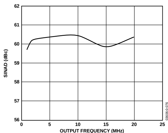
Figure 47. AD9861 Tx Path SINAD vs. Output Frequency of Tx Path, with 20 mA Full-Scale Output into 60 \Omega Differential Load
