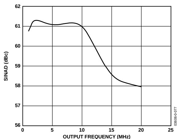
Figure 50. AD9861 Tx Path SINAD vs. Output Frequency of Tx Path, with 2 mA Full-Scale Output into 600 \Omega Differential Load
