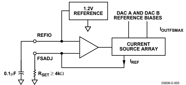
Figure 74. Reference Circuitry
