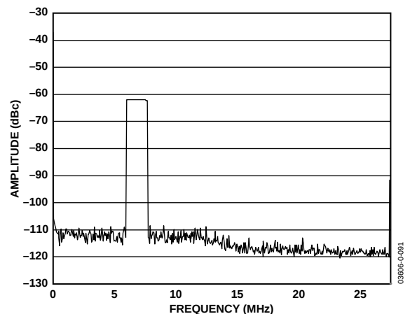
Figure 63. AD9861 Tx Path FFT of OFDM Signal in Figure 52, with 4 \times Interpolation
