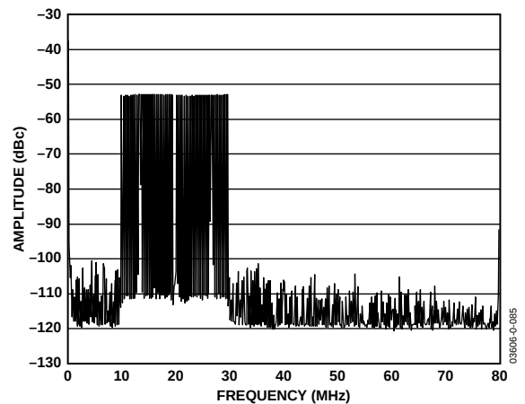
Figure 57. AD9861 Tx Path FFT of OFDM Signal in Figure 52, with 4 \times Interpolation
