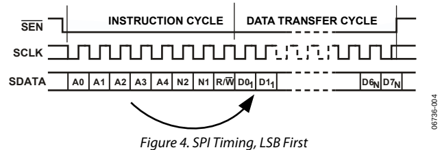
Figure 4. SPI Timing, LSB First
