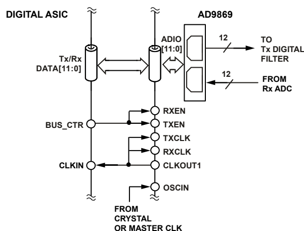
Figure 11. Example of a Half-Duplex Digital Interface with AD9869 Serving as the Master
