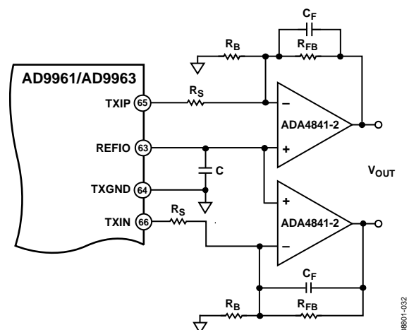
Figure 62. Single-Supply Differential Buffer
