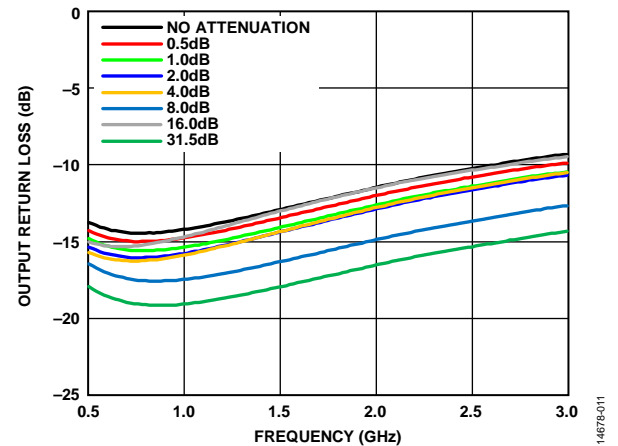
Figure 12. Output Return Loss vs. Frequency, Major States Only
