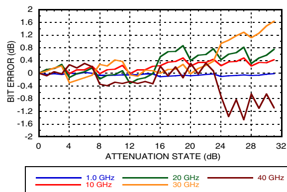
Bit Error vs. Attenuation State
