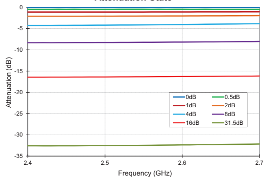
Normalized Attenuation versus Frequency and Attenuation State
