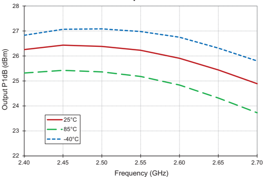
Output P1dB versus Frequency and Temperature
