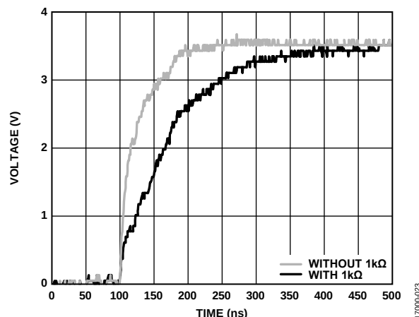
Figure 23. Using a Resistor on SEROUT
