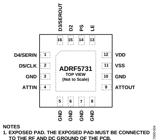
Figure 4. Pin Configuration
