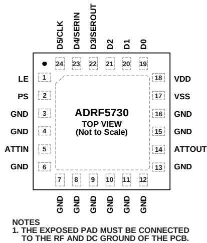
Figure 4. Pin Configuration
