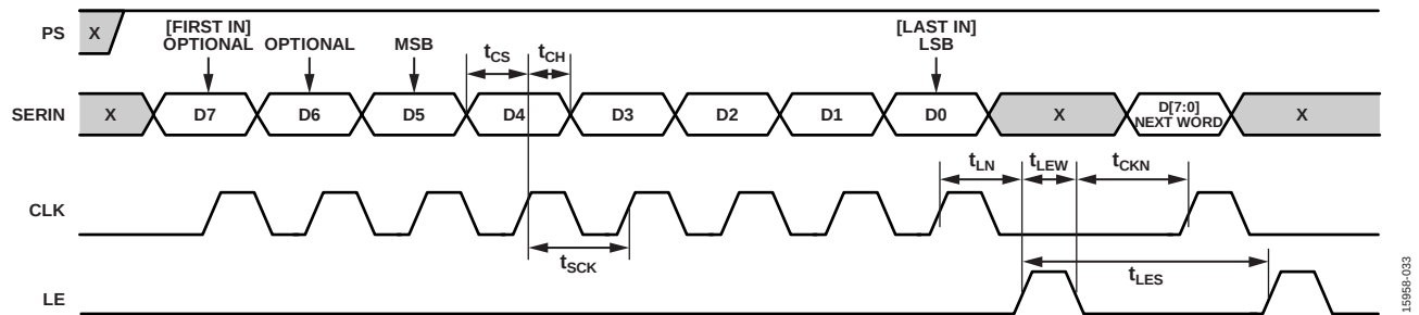
Figure 34. Serial Control Timing Diagram
