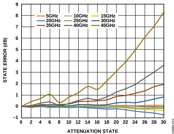
Figure 15. State Error vs. Attenuation State over Frequency
