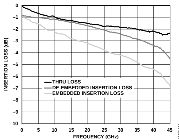
Figure 28. Insertion Loss vs. Frequency
