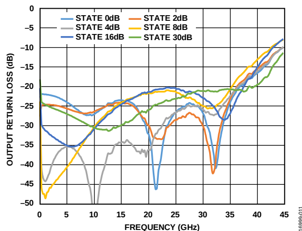
Figure 11. Output Return Loss vs. Frequency (Major States Only)
