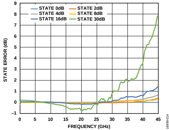
Figure 14. State Error vs. Frequency (Major States Only)
