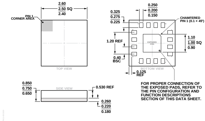
Figure 34. 16-Terminal Land Grid Array [LGA] 2.5 mm × 2.5 mm Body and 0.75 mm Package Height (CC-16-6) Dimensions shown in millimeters
