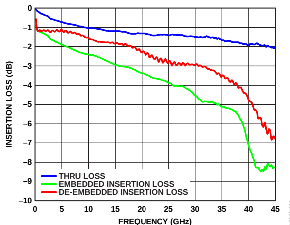
Figure 38. Insertion Loss vs. Frequency
