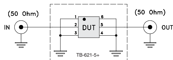
Fig 1. Block diagram of Test Circuit used for characterization, Test board TB-621-5+ Conditions: Attenuation, VSWR: Pin=-10 dBm
